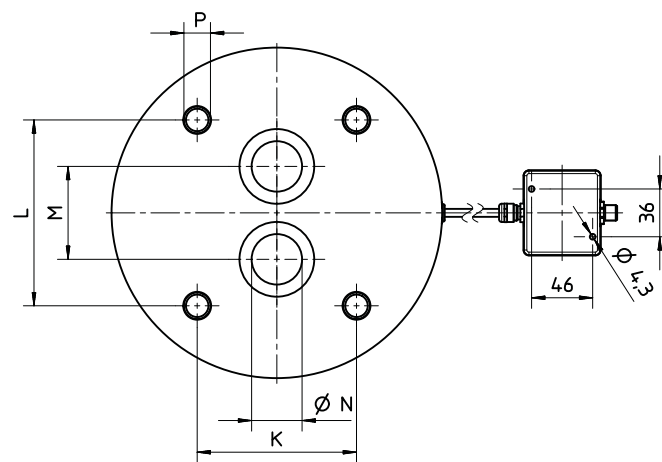
Connection dimensions
