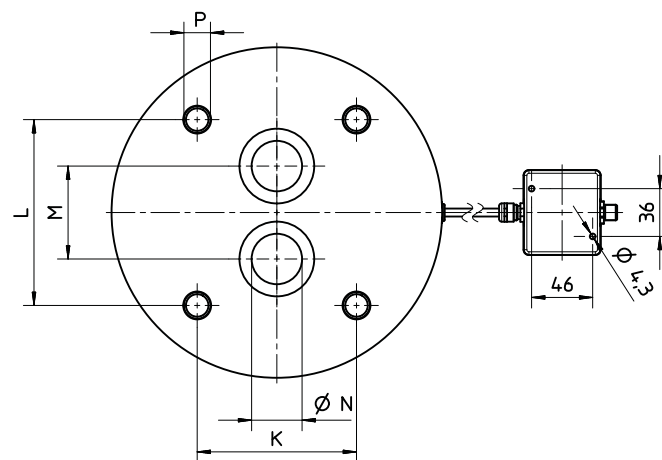
Connection dimensions
