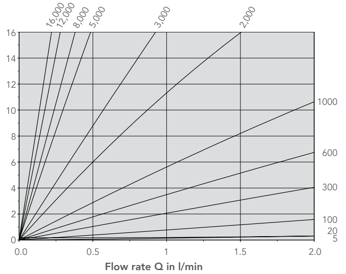
VC 0.2 (section)
